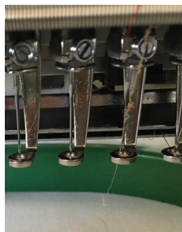
Figure 2 Violation of sewing hybrid thread in the middle of embroidering process
